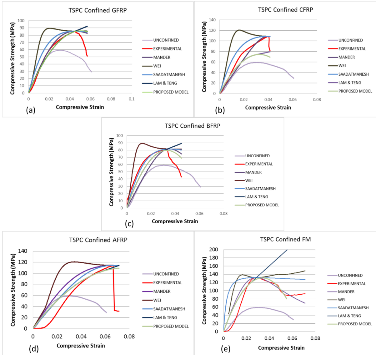
Figure 6: Stress versus strain curve of experimental and mathematical prediction. (a) TSPC confined GFRP (TSPC-GF). (b) TSPC confined CFRP (TSPC-CF). (c) TSPC confined BFRP (TSPC-BF). (d) TSPC confined AFRP (TSPC-AF). (e) TSPC confined mild steel tube (TSPC-FM).
