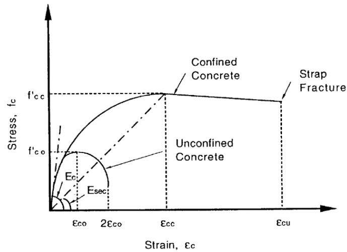
Figure 2: Stress versus strain model of confined concrete strength based on Saadatmanesh et. al 1994
