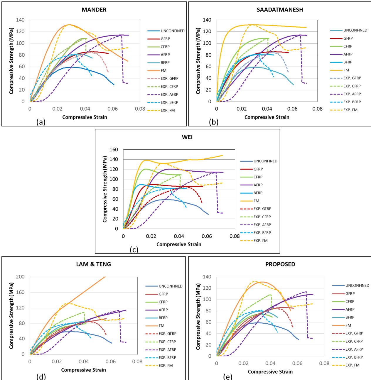
Figure 7: Stress versus strain curve of all confined TSPC samples by experimental and mathematical prediction. (a) Mander model. (b) Saadatmanesh model. (c) Wei model. (d) Lam & Teng model. (e) Proposed model.
